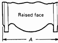
Class 250 Cast Iron and Class 300 Steel
