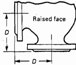
Class 250 Cast Iron and Class 300 Steel
